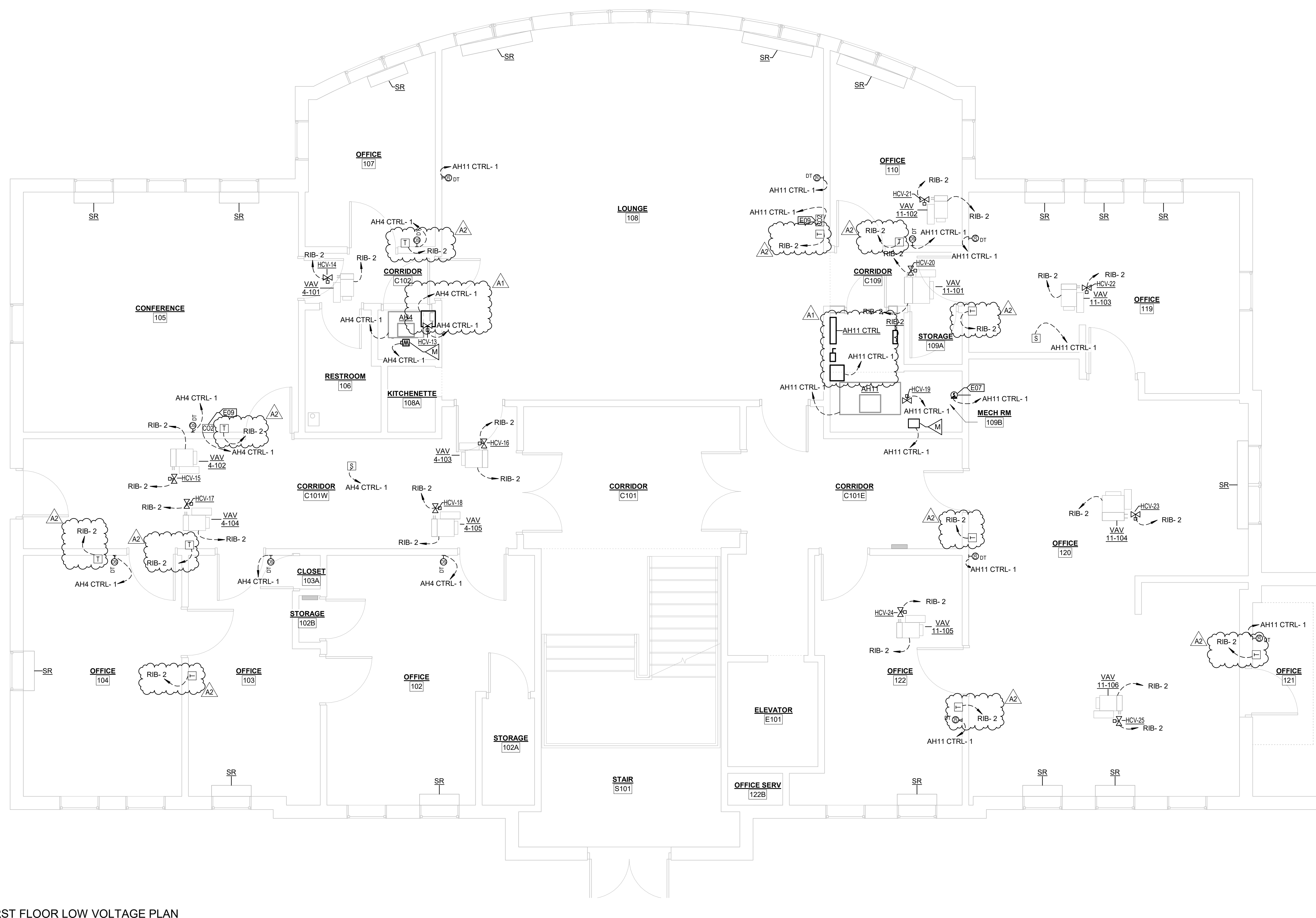
1 FIRST FLOOR LOW VOLTAGE PLAN 1/4" = 1'-0"
